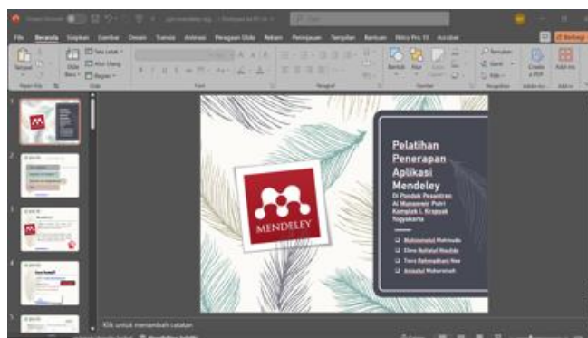
Gambar 1. Materi Mendeley
