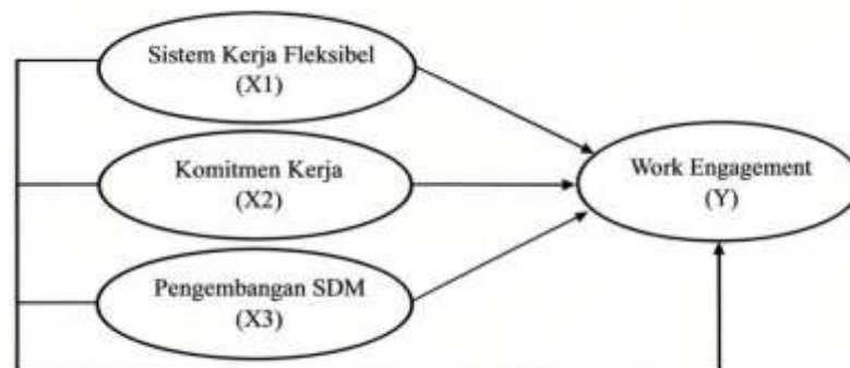
Gambar 1. Model Penelitian
